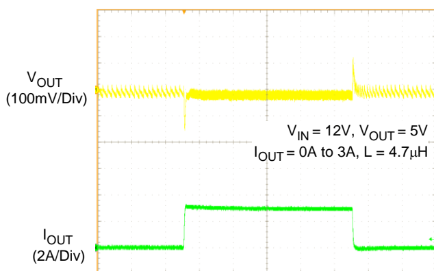
Time (200µs/Div)
