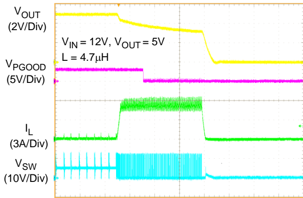
Time (50μs/Div)
