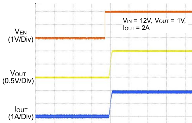
Time (4ms/Div)
