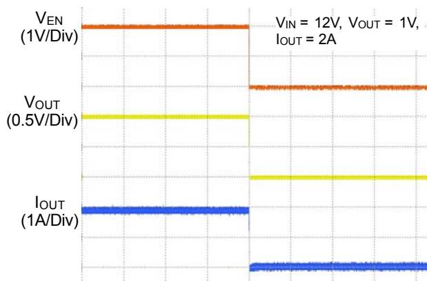
Time (4ms/Div)
