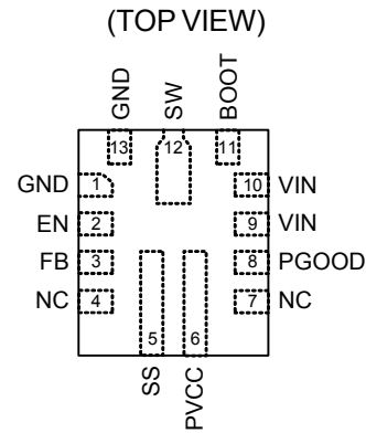
UQFN-13JL 2x3 (FC)
