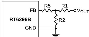
Figure 1. Output Voltage Setting
