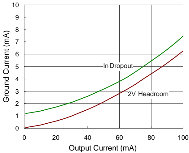
Ground Current vs. Output Current
