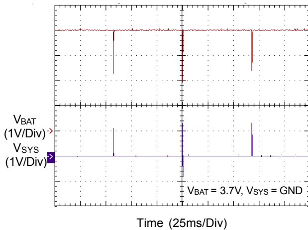
V_{SYS} Short to GND Protection with Battery
