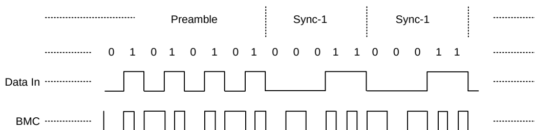
Figure 4. BMC Example
