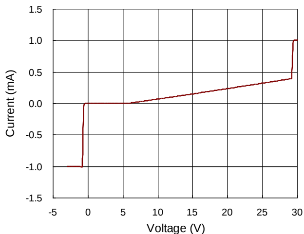
CON_CC IV Curve
