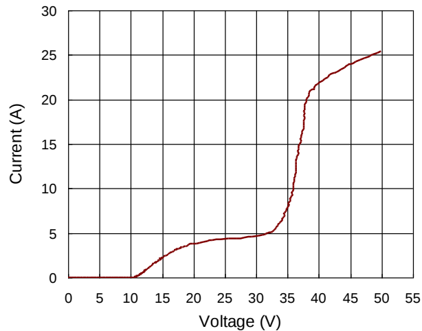
CON_CC TLP Curve Unpowered
