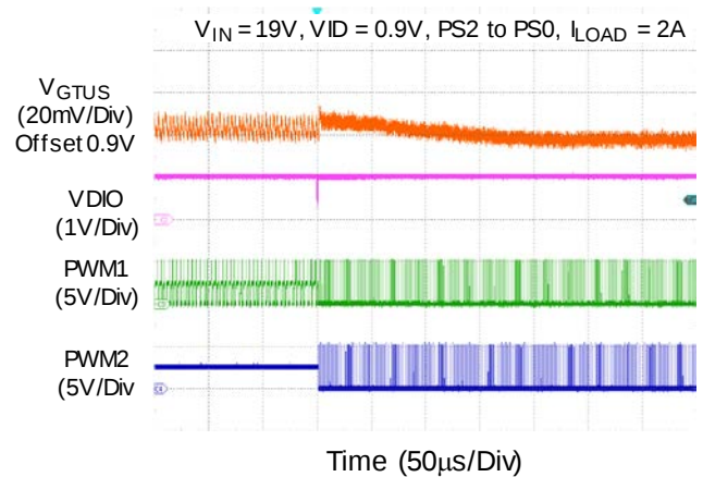
GTUS VR Mode Transient
