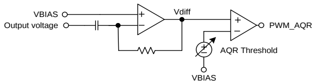
Figure 19. Adaptive Quick Response Mechanism
