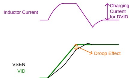
Figure 15. Droop Effect in VID Transition
