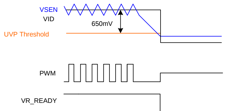
Figure 25. Under-Voltage Mechanism
