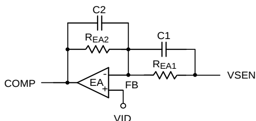
Figure 17. Type I Compensator
