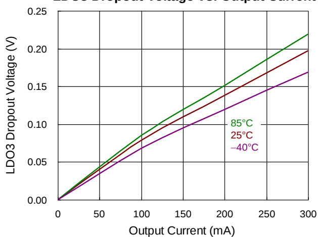
LDO3 Dropout Voltage vs. Output Current
