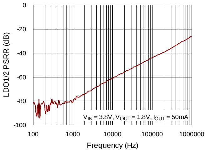
LDO1/2 PSRR
