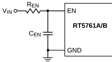
Figure 7. Enable Timing Control
