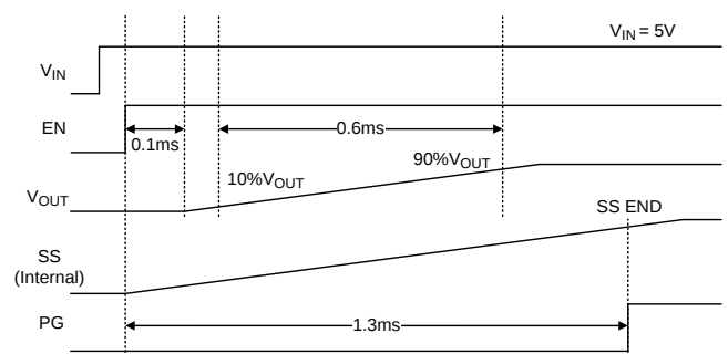
Figure 1. Start-Up Sequence
