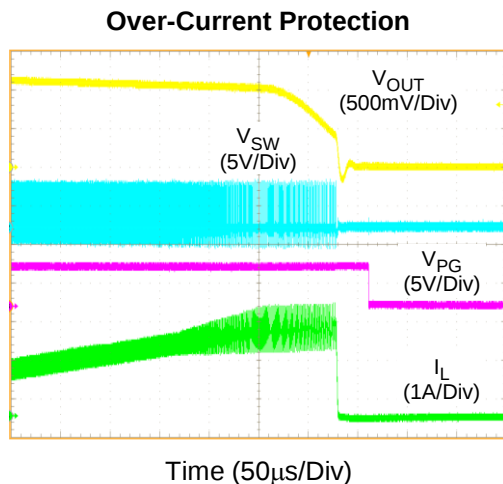
Figure 3. Over-Current Protection
