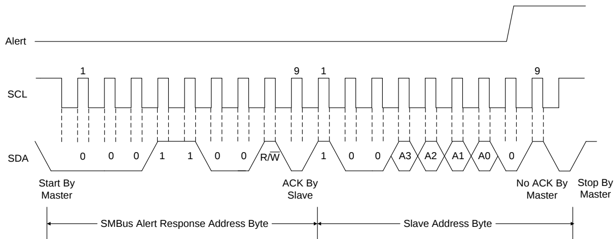
Figure 6. Timing Diagram for SMBus Alert
