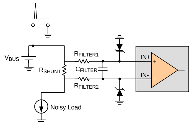
Figure 8. RT6053 with Input Protection
