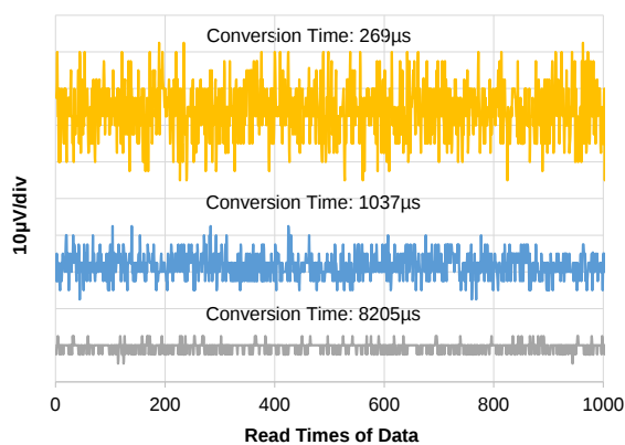
Figure 1. Noise vs Conversion Time
