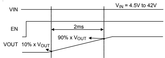
Figure 1. Start-Up Sequence
