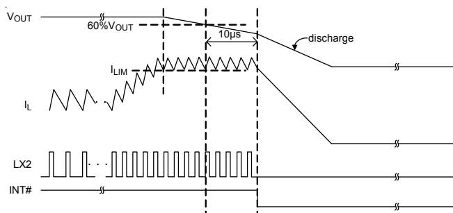
Figure 11. Current-Limit Behavior
