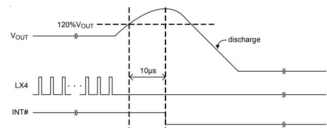
Figure 15. OVP Behavior
