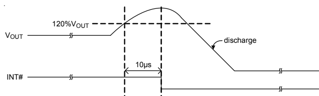
Figure 19. OVP Behavior
