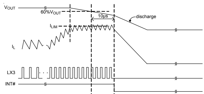
Figure 14. Current-Limit Behavior
