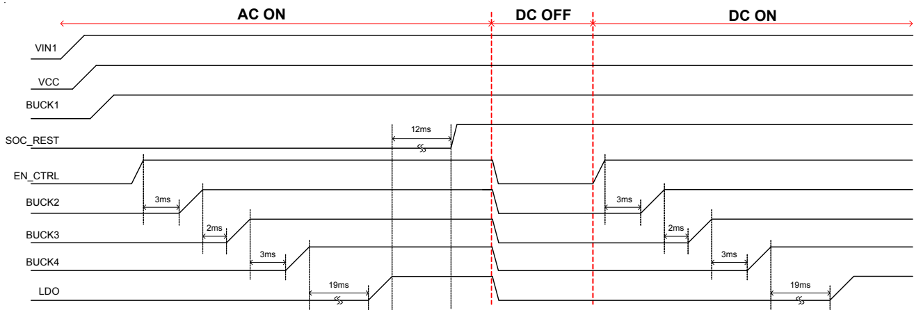
Figure 3. Power-ON Sequence
