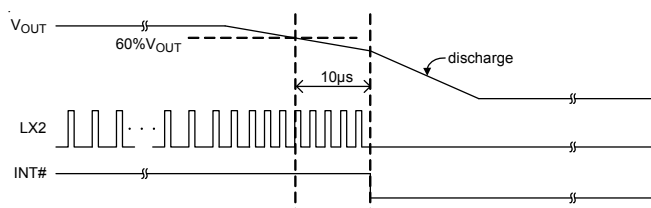
Figure 10. UVP Behavior
