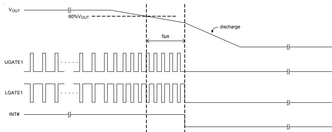
Figure 7. UVP Behavior
