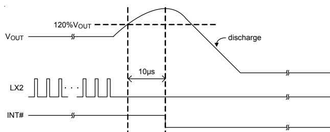
Figure 9. OVP Behavior
