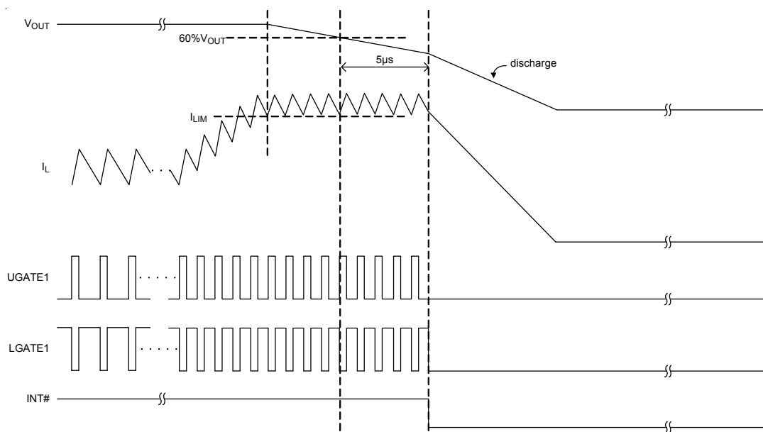
Figure 5. Current-Limit Behavior
