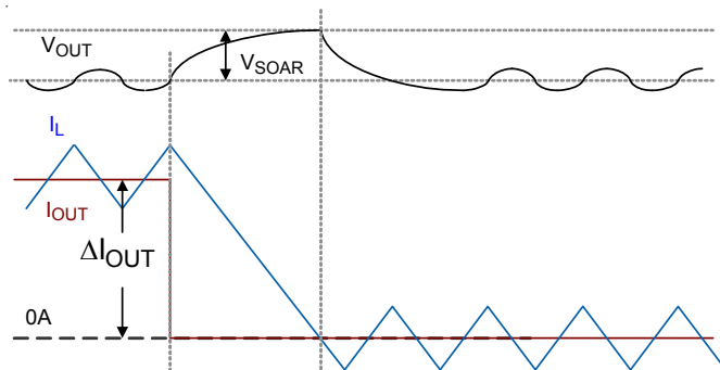
Figure 8. Output Voltage SOAR ( V_{SOAR} ) Estimation as Output Load Current Step Down
