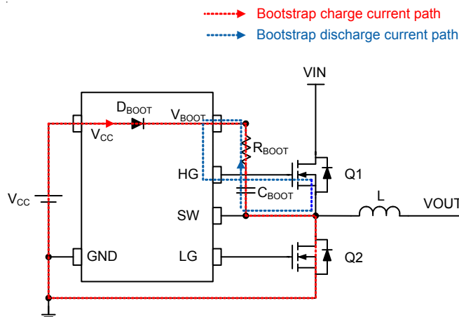
Figure 11. Bootstrap Power Supply Circuit
