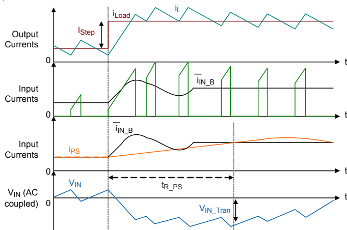
Figure 10. VIN Transient Current Diagram
