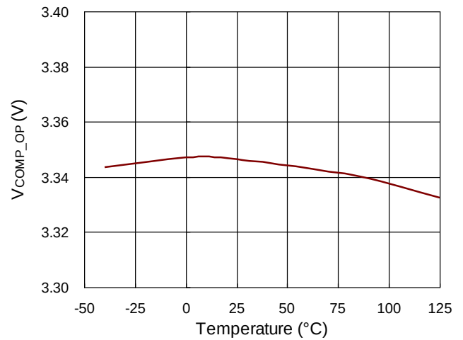
V COMP_OP vs. Temperature
