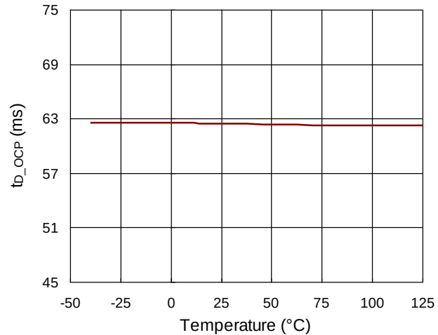
t_{D\_OCP} vs. Temperature
