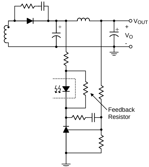
Figure 9. Feedback Resistor
