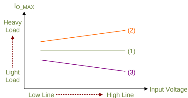
Figure 6. Output Current Limits for Over-Current Protection
