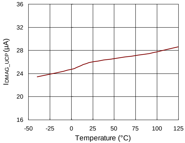
I DMAG_UCP vs. Temperature
