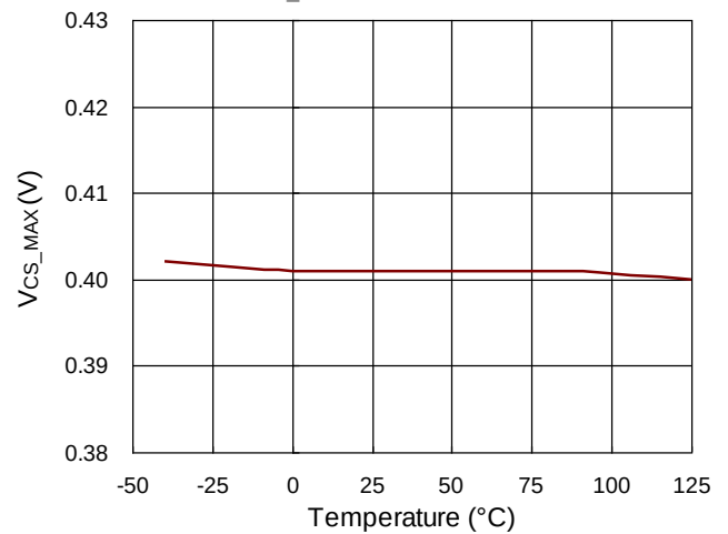
V CS_MAX vs. Temperature
