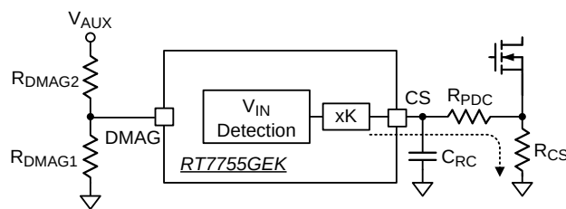
Figure 5. Functional Block Diagram of Line Compensation
