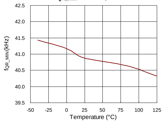
f QR_MIN vs. Temperature
