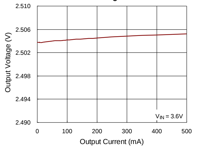
Load Regulation
