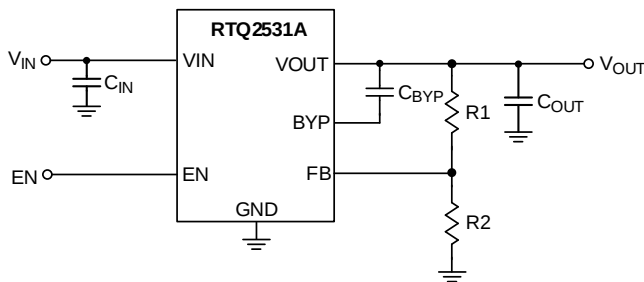
Figure 1. Output Voltage Set by External Resistors
