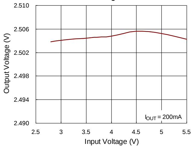
Line Regulation
