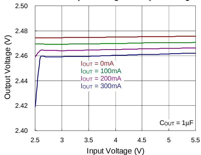
LDO7 Output Voltage vs. Input Voltage
