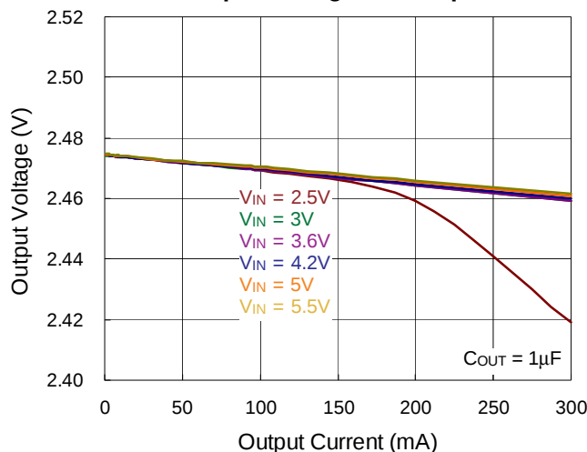
LDO7 Output Voltage vs. Output Current
