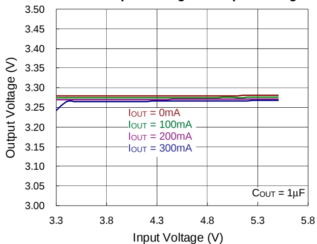
LDO5 Output Voltage vs. Input Voltage
