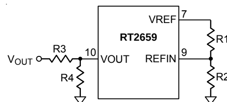
Figure 8. VCC = 3V and High V OUT Application Setting
