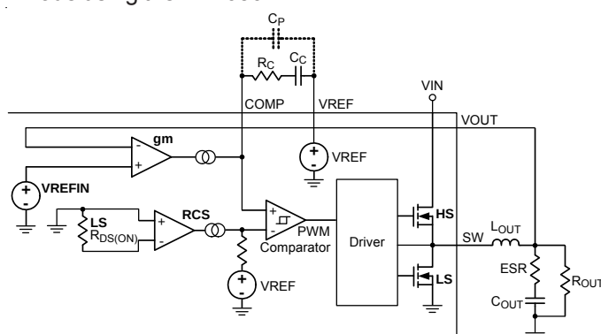
Figure 2. Non-Droop Mode
