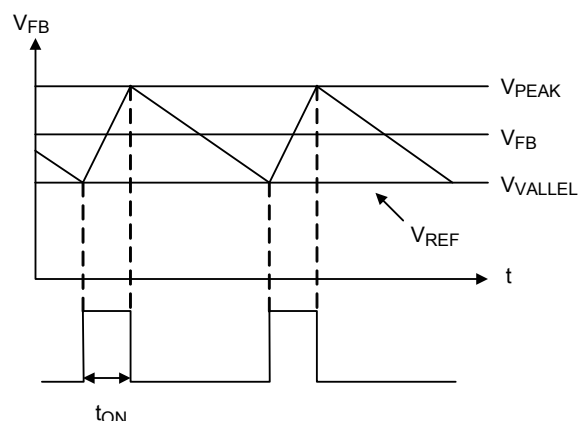
Figure 1. Constant On-Time PWM Control
