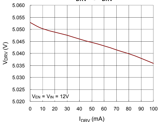
VDRV vs. IDRV
