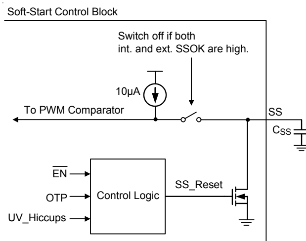
Figure 3. Soft-Start Control Block.
