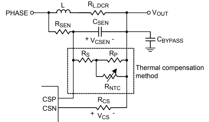
Figure 8. Thermal Compensation Method
