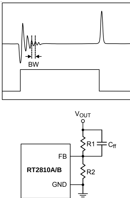
Figure 1. C_{\text{ff}} Capacitor Setting
