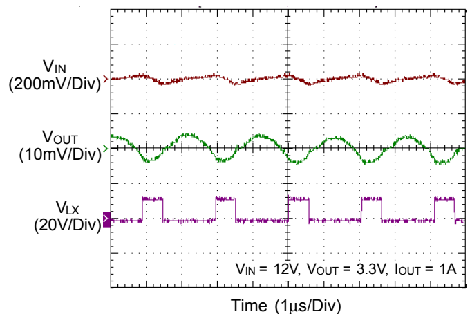
Voltage Ripple
