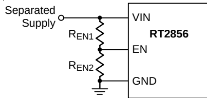
Figure 5. Resistor Divider for VIN UVLO Setting, V_{IN} \geq 4.5V
