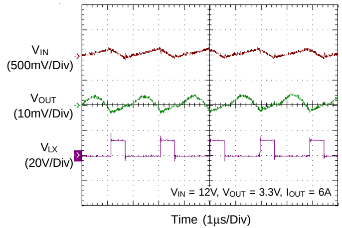
Voltage Ripple
