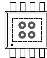
Figure 8. Standard PTH to GND Plane
