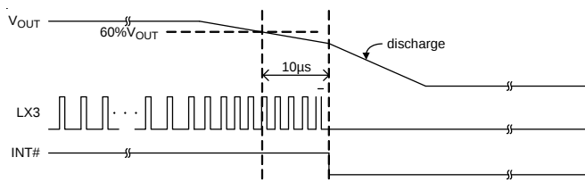
Figure 13. UVP Behavior
