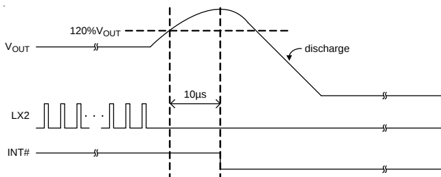
Figure 9. OVP Behavior
