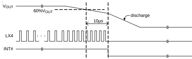
Figure 16. UVP Behavior
