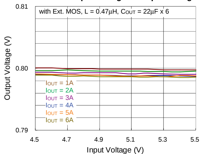
BUCK3 Output Voltage vs. Input Voltage
