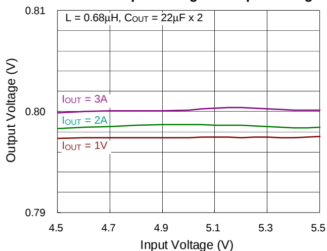
BUCK2 Output Voltage vs. Input Voltage
