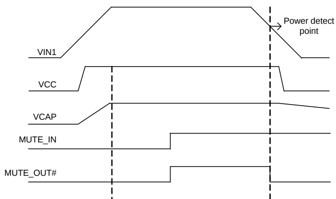
Figure 22. Mute Sequence when AC OFF in 24V Single Input Power System
