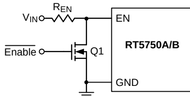
Figure 8. Logic Control for the EN Pin
