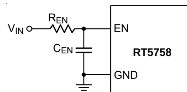
Figure 3. Enable Timing Control
