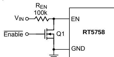
Figure 4. Logic Control for the EN Pin
