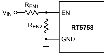
Figure 5. Resistive Divider for Under-Voltage Lockout Threshold Setting
