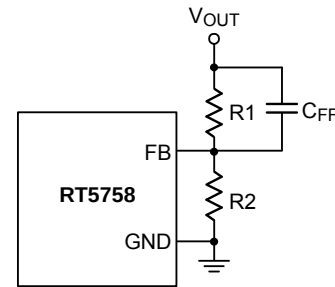
Figure 2. C_{FF} Capacitor Setting
