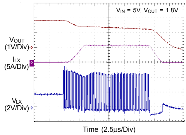
Over-Current Protection
