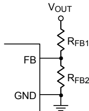
Figure 1. Setting V_{OUT} with a Voltage Divider
