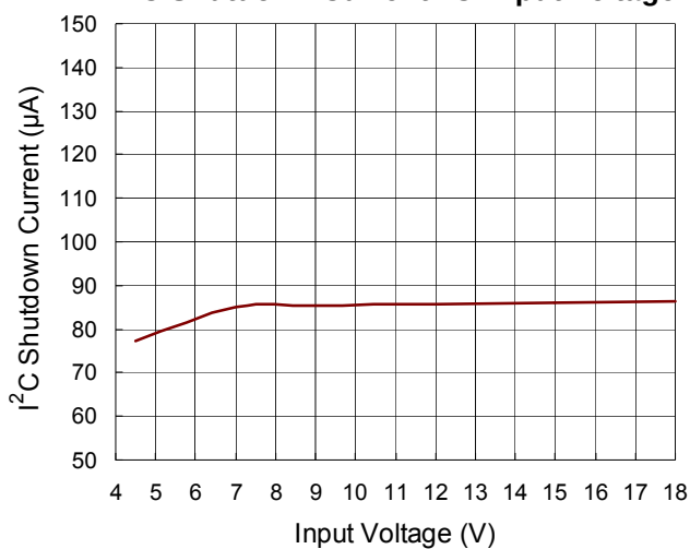
I 2 C Shutdown Current vs. Input Voltage
