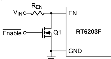
Figure 3. Logic Control for the EN Pin
