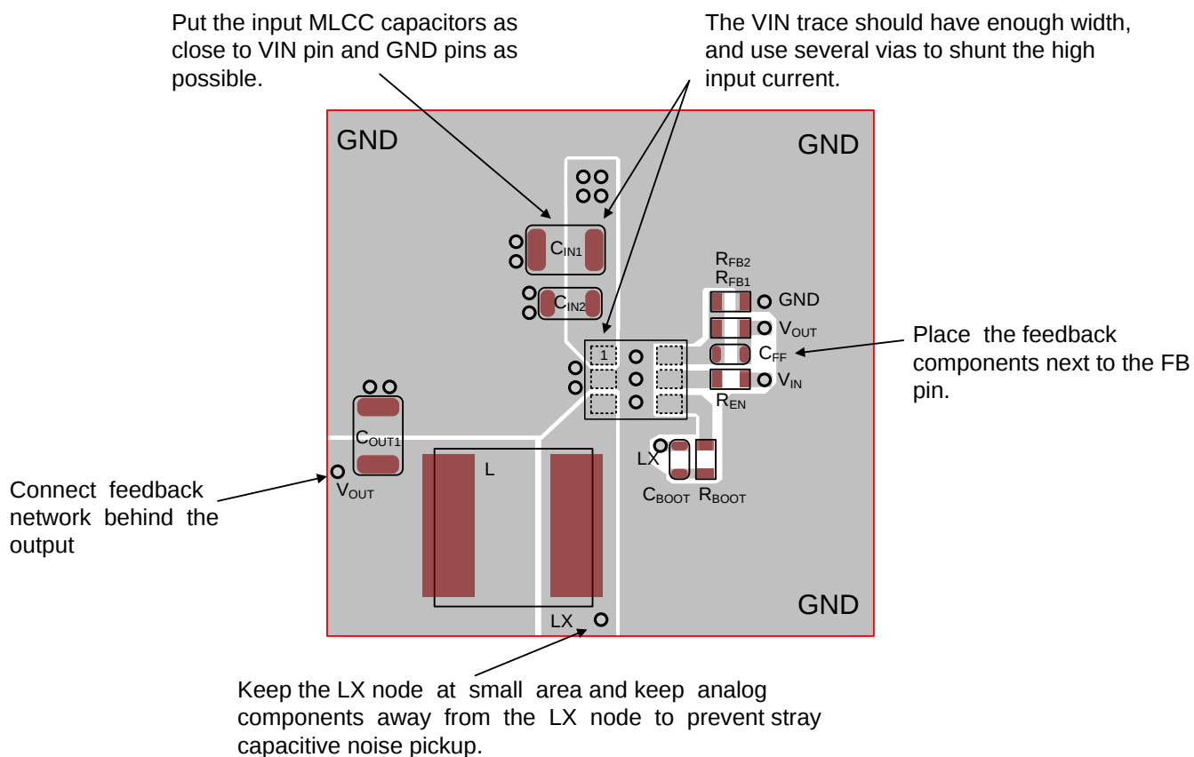
Figure 8. PCB Layout Guide
