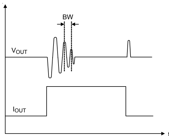
Figure 8. A Simply Way to Get the Bandwidth
