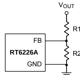
Figure 5. Output Voltage Setting
