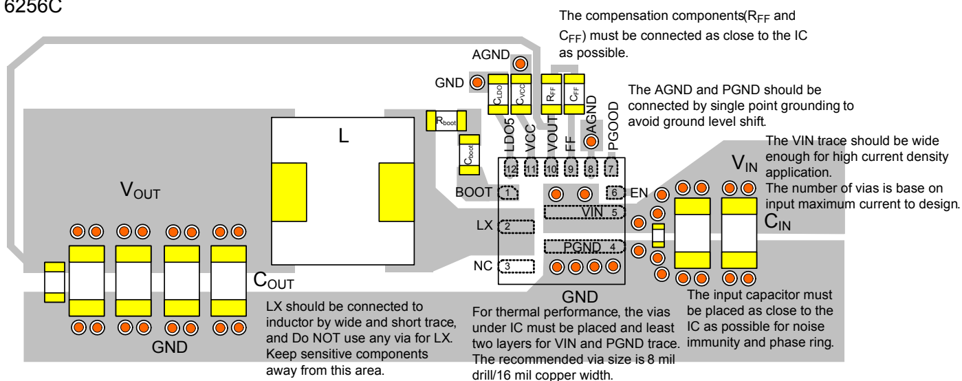
Figure 9. Layout Guide of RT6256C
