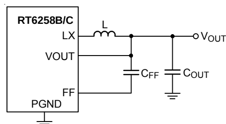
Figure 4. Feedback Loop with Feedforward Capacitor
