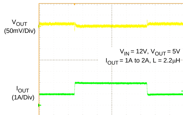
Load Transient (Half Load to Full Load)
