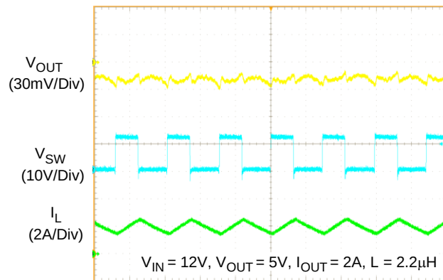
Output Ripple as I_{OUT} = 2A
