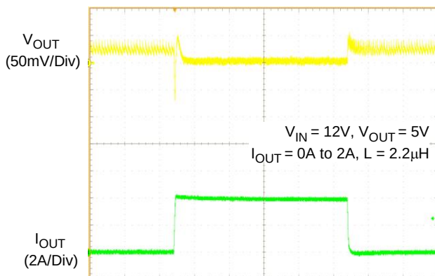
Load Transient (No Load to Full Load)
