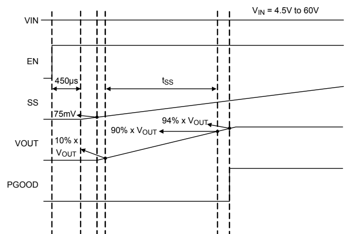
Figure 1 Start-Up Sequence for RT6362GQW and RT6362GFP
