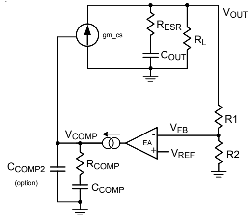
Figure 9. Simplified Equivalent Circuit of Buck with PCCM
