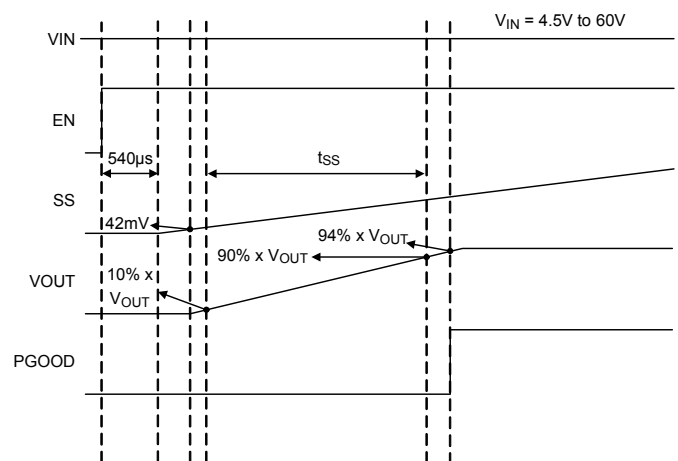
Figure 1 Start-Up Sequence for RT6363GQW
