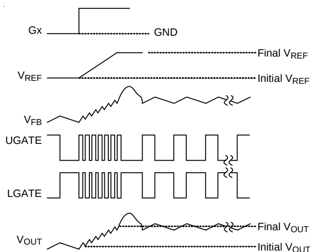
Figure 4. Output Voltage Up Transition with Overshooting
