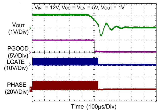
Under-Voltage Protection
