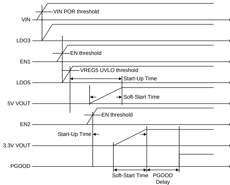
Figure 5. RT6576C Timing
