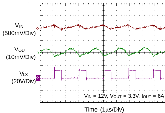
Voltage Ripple
