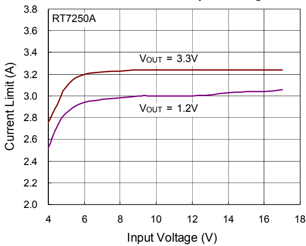
Current Limit vs. Input Voltage
