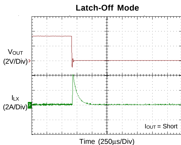
Figure 6. Latch-Off Mode Under Voltage Protection
