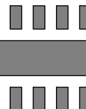
(c) Copper Area = 30 \text{ mm}^2 , \theta_{JA} = 54^\circ\text{C/W}
