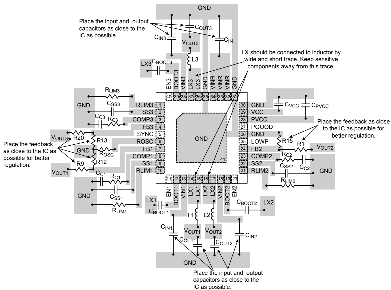
Figure 10. PCB Layout Guide
