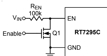
Figure 3. Digital Enable Control Circuit
