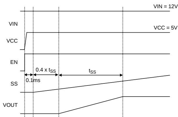
Figure 1 Start-Up Sequence
