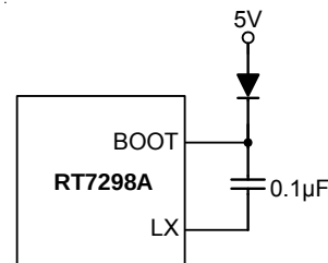
Figure 9. External Bootstrap Diode
