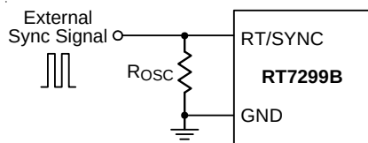
Figure 8. External Sync Signal Control
