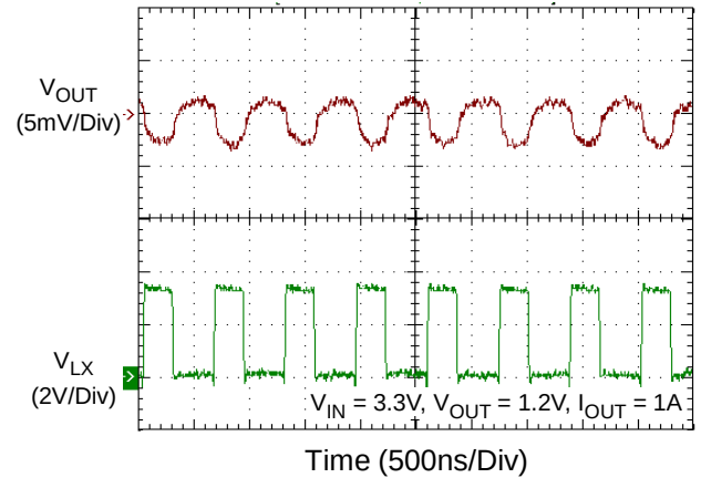
Voltage Ripple
