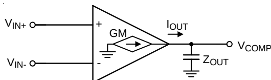
Figure 2. Operational Transconductance Amplifier, EOTA
